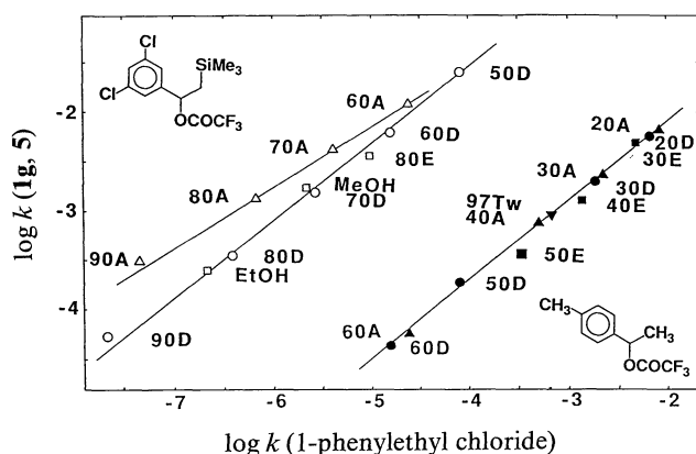
Fig. 1. Plots of \log k for 1g (open circles, triangles, and squares) and 5 (closed circles, triangles, and squares) vs. \log k (1-phenylethyl chloride 3b ) in various solvents.
